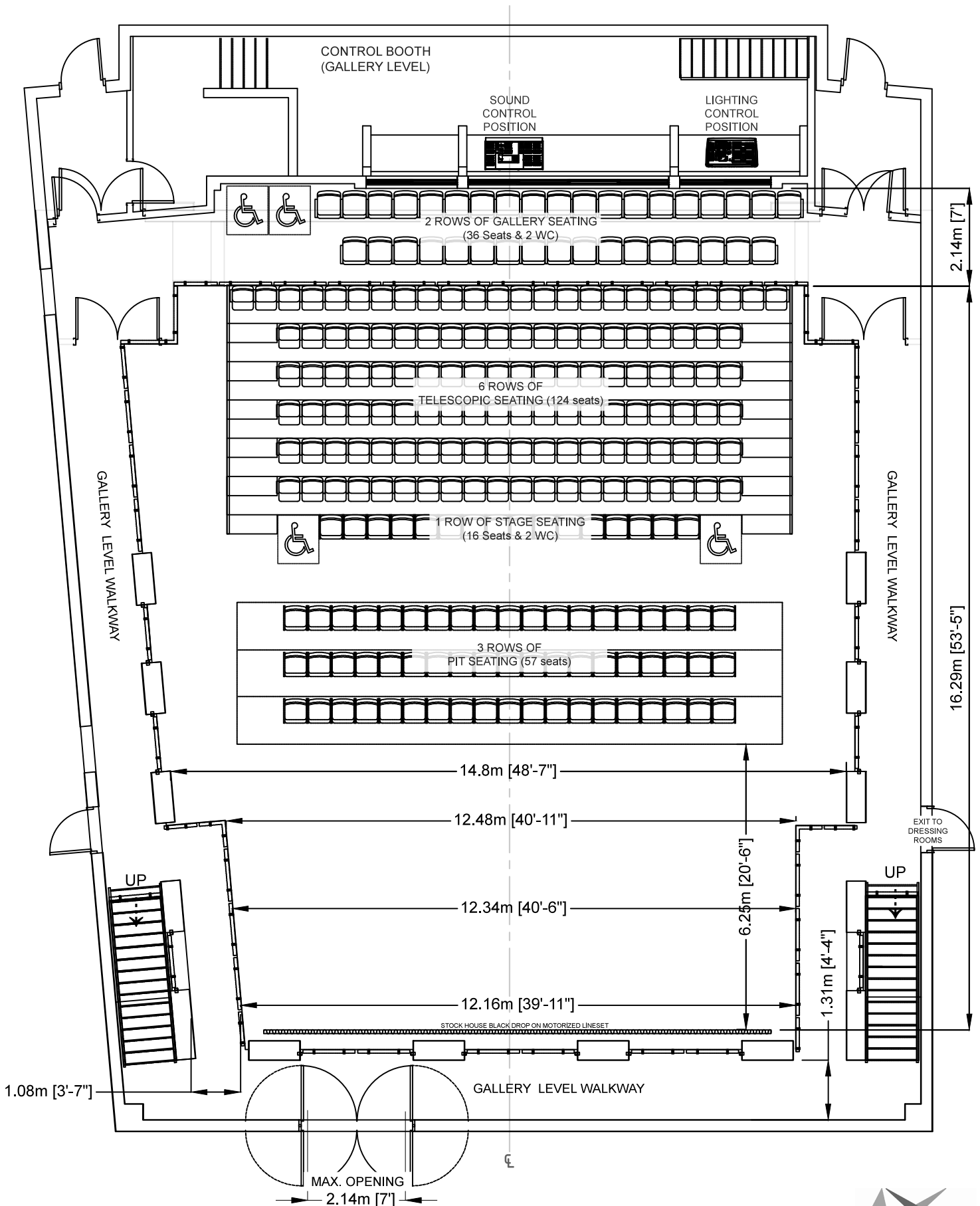
CentrepoinTE Studio Theatre Floor Plan - Pit Seating Configuration
